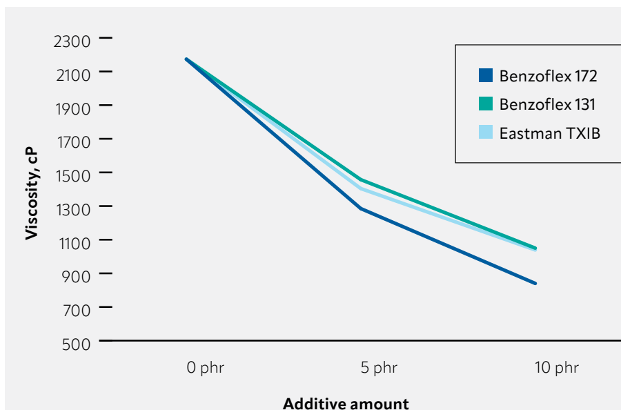
Figure 1. Viscosity reduction
