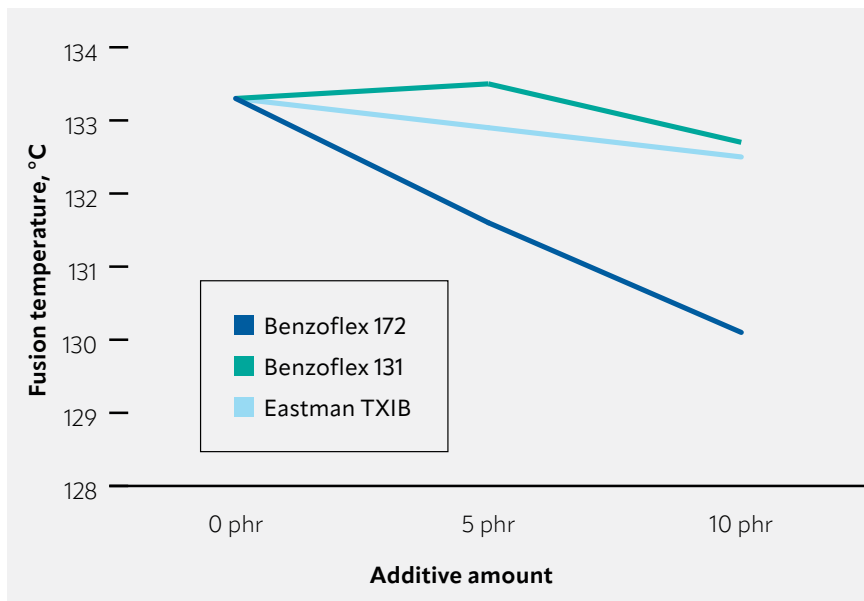
Figure 3. Solvating power
