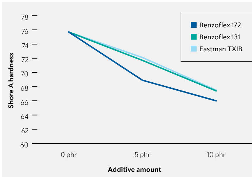
Figure 2. Plasticizer efficiency
