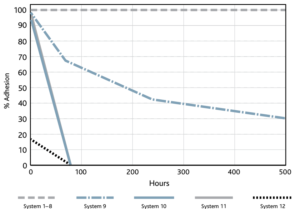
Figure 1 Humidity resistance of CPO primers a,b % Retained adhesion
